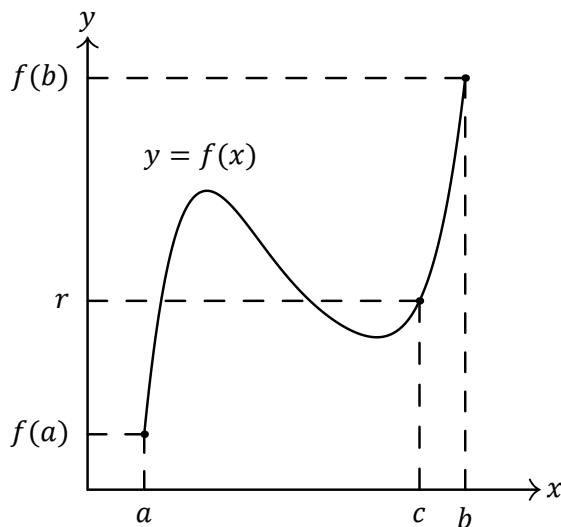
Figure 6.1: The intermediate value theorem.
