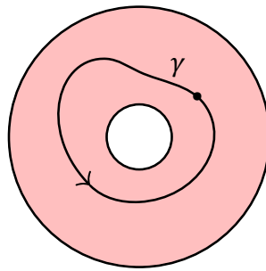
Figure 1.3: A loop.
