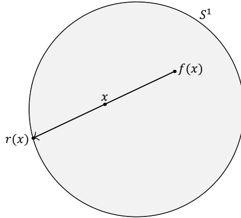
Figure 8.3: The map r: D^2 \rightarrow S^1 .
