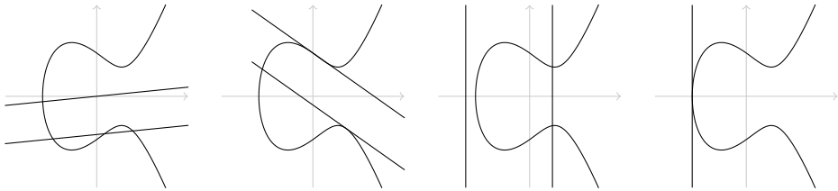
Figure 4: Intersection of lines and elliptic curves. From left to right: three distinct intersection points, possibly with complex Y -coordinates; tangent lines with one or two distinct intersection points; two distinct intersection points, possibly with complex Y -coordinates; and a tangent line with one intersection point.
