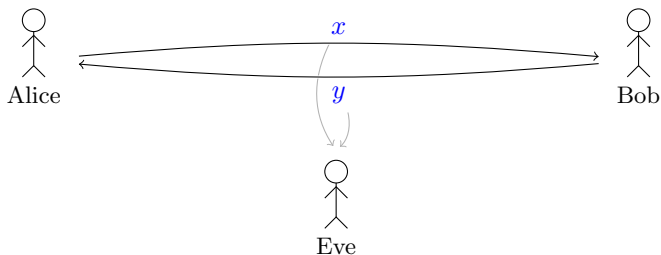
Figure 2: Eve is listening and learns x and y , but cannot see Alice's and Bob's secret values or computations. She already knows G , g and n .
