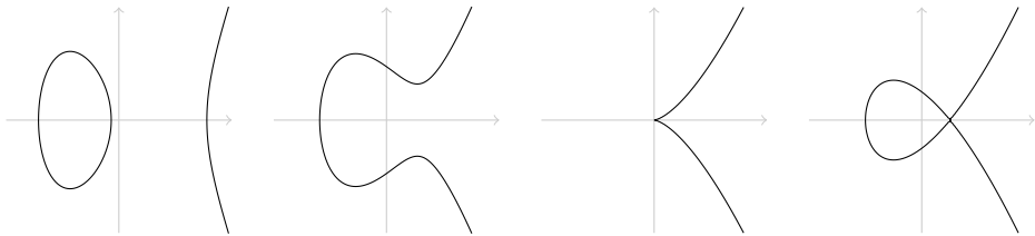
Figure 3: Four cubic curves. From left to right: Y^2 = X^3 - 6X - 1 , Y^2 = X^3 - 2X + 2 , Y^2 = X^3 and Y^2 = X^3 - \frac{3}{4}X + \frac{1}{4} .
