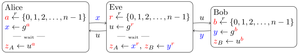
Figure 5: A man-in-the-middle attack on the Diffie-Hellman protocol, where Eve establishes separate shared secrets with Alice and Bob, who do not notice the attack.
