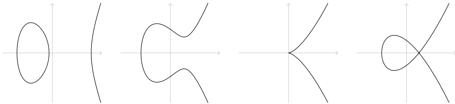
Figure 2: Four cubic curves. From left to right: Y^2 = X^3 - 6X - 1 , Y^2 = X^3 - 2X + 2 , Y^2 = X^3 and Y^2 = X^3 - \frac{3}{4}X + \frac{1}{4} .
