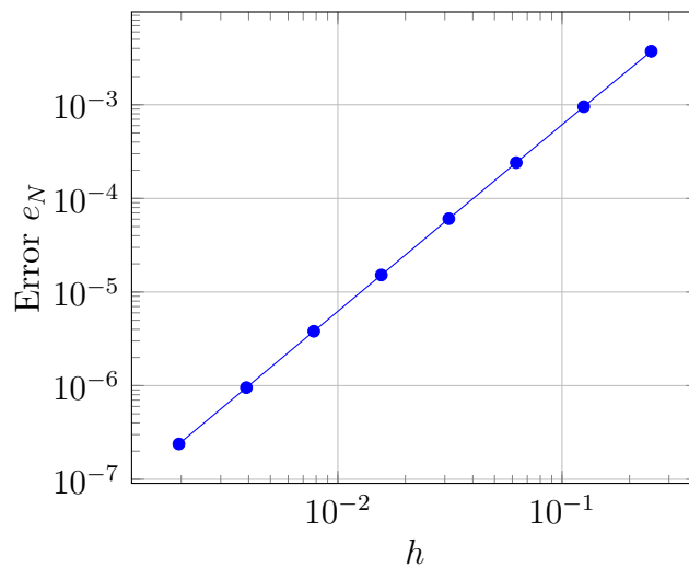
Convergence plot
